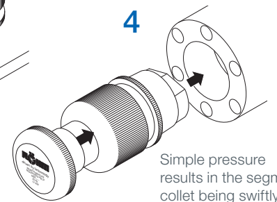
Pre-positioning of the segment collet
